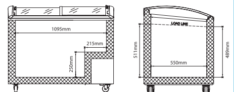
F38 Internal Dimensions
